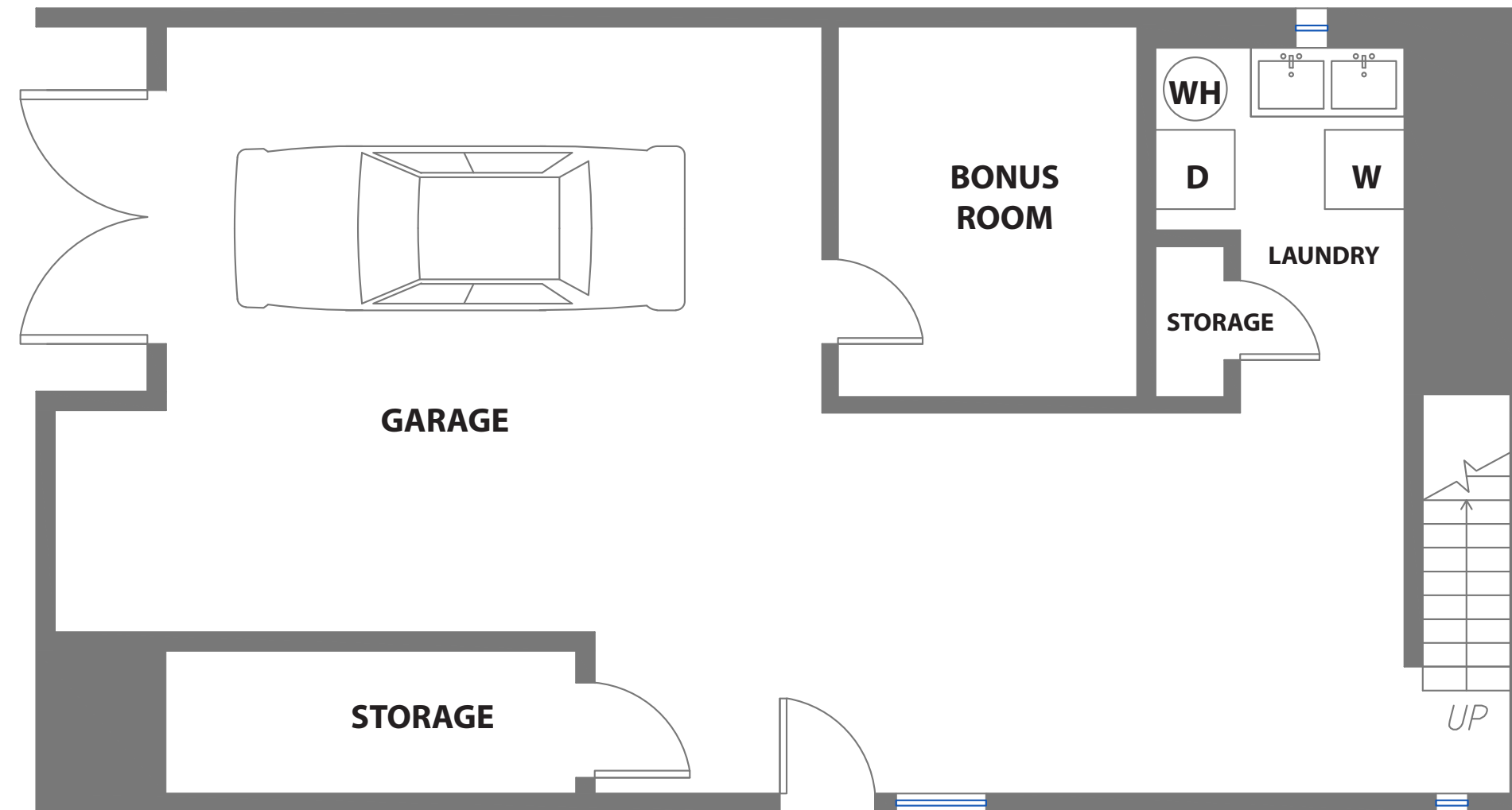
GARAGE
